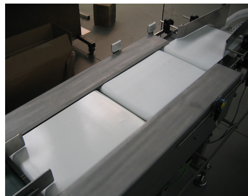
Photo: dynamic belt infeed
