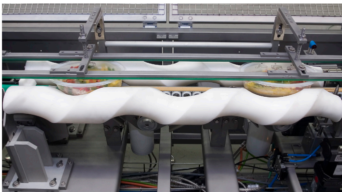
Photo: worm infeed
