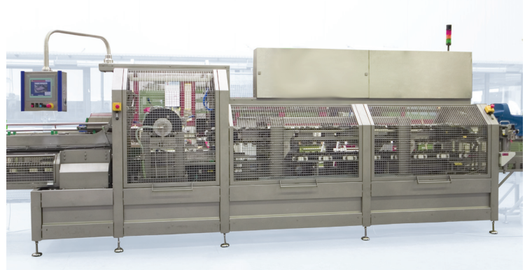
Sleeve-Maschine BM150 Sleeve Machine BM150
